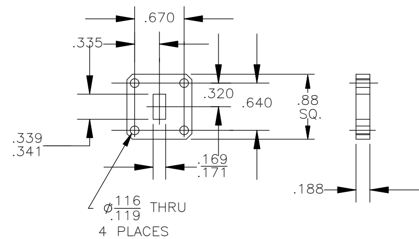
DETAIL: "A" WR34 FLANGE, COVER TOLERANCES: 2 PLACES - ±.01 3 PLACES - ±.005
